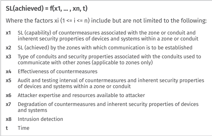
Figure 4. Required Factors to Reach IEC 62443's SL-A
