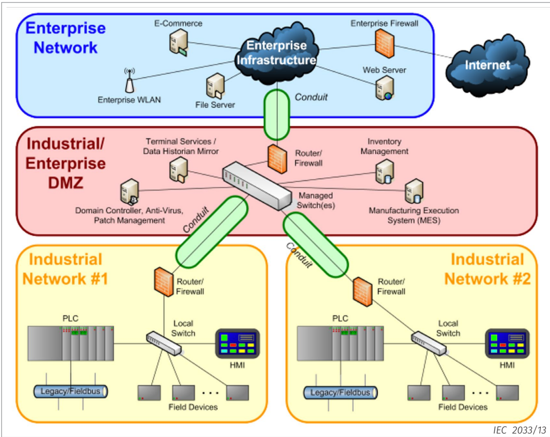
Figure 7. High-Level Manufacturing Example Showing Zones and Conduits
